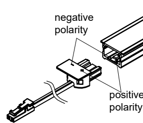
SY2480M middle connector
